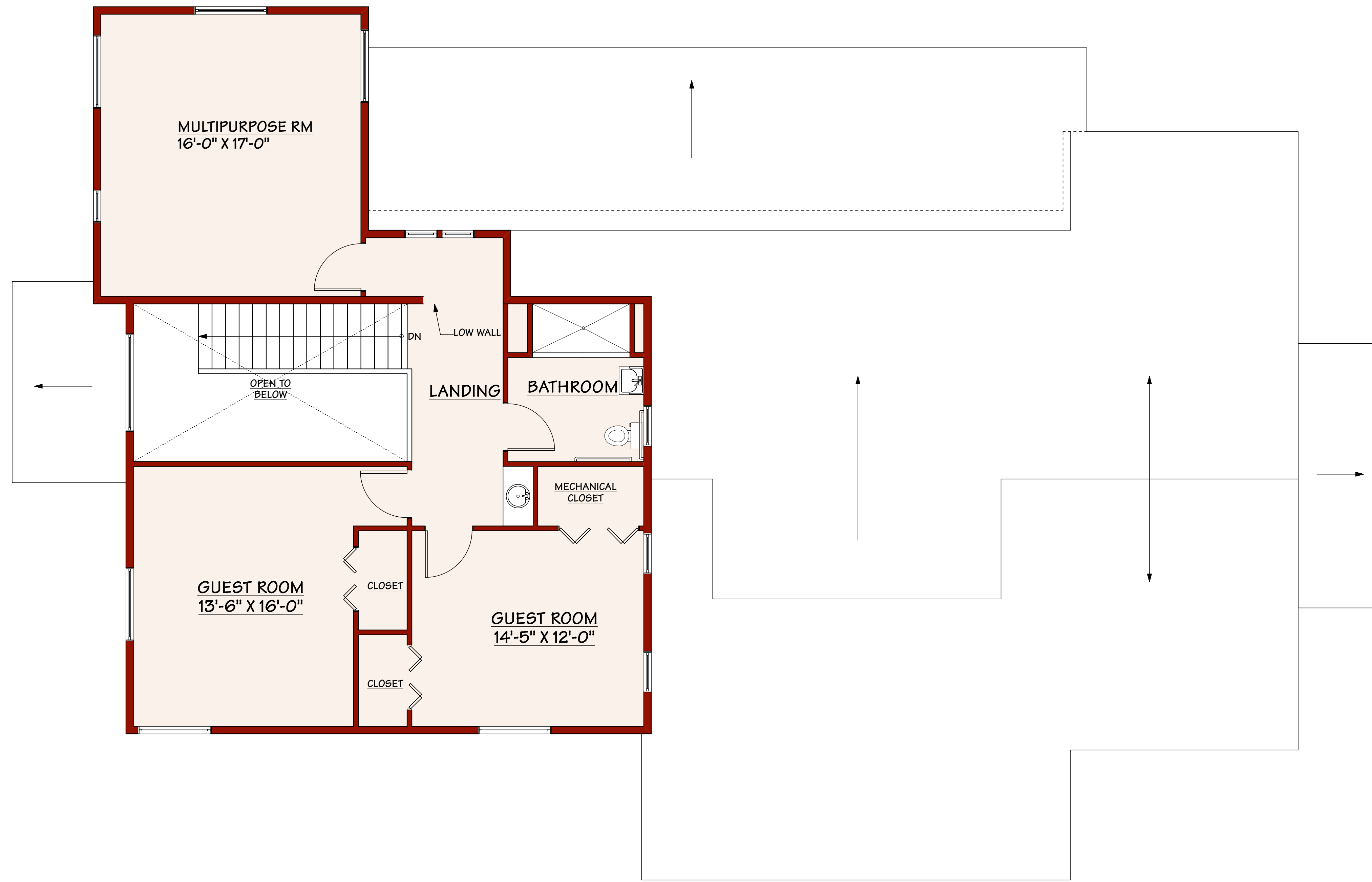
SECOND FLOOR PLAN 1,040 SF
