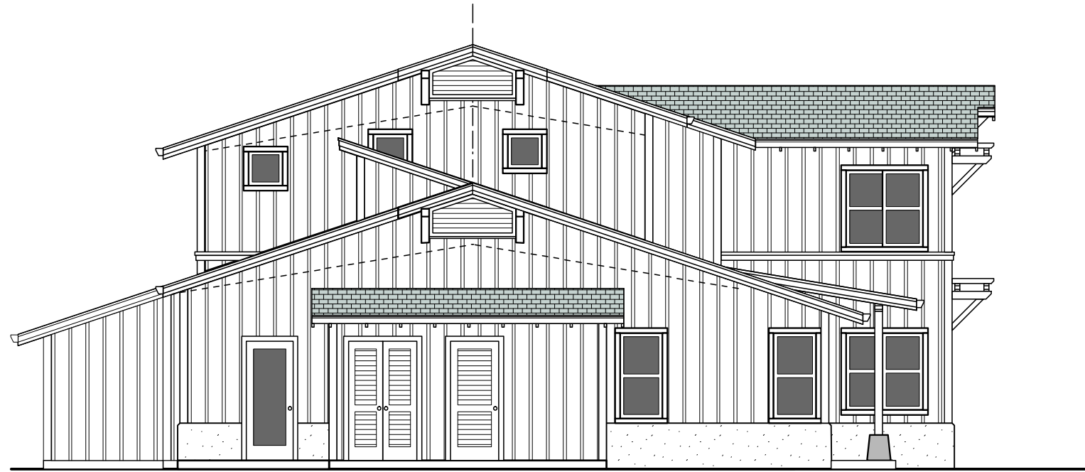
4 NORTH ELEVATION Scale: 1/4"=10' (@24"x36" PAPER SIZE)
